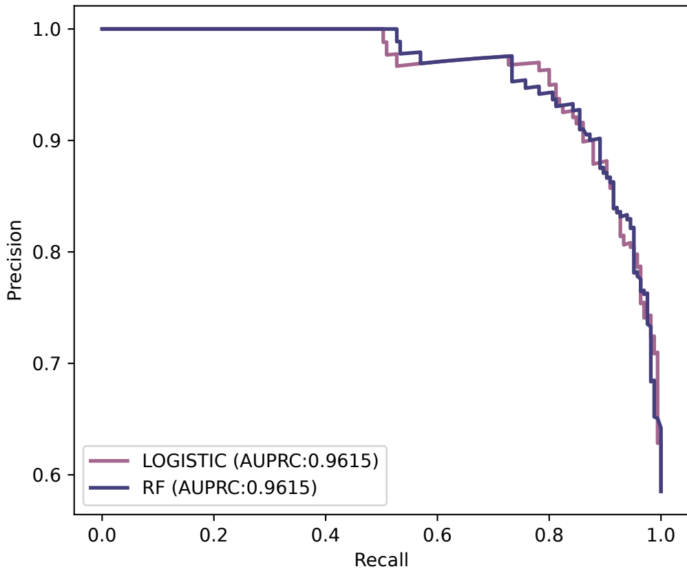
PR Curves of Multiple Models
